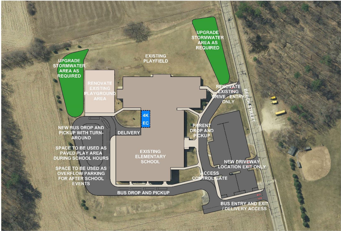
1 ELEMENTARY SCHOOL SITE FLOOR PLAN
